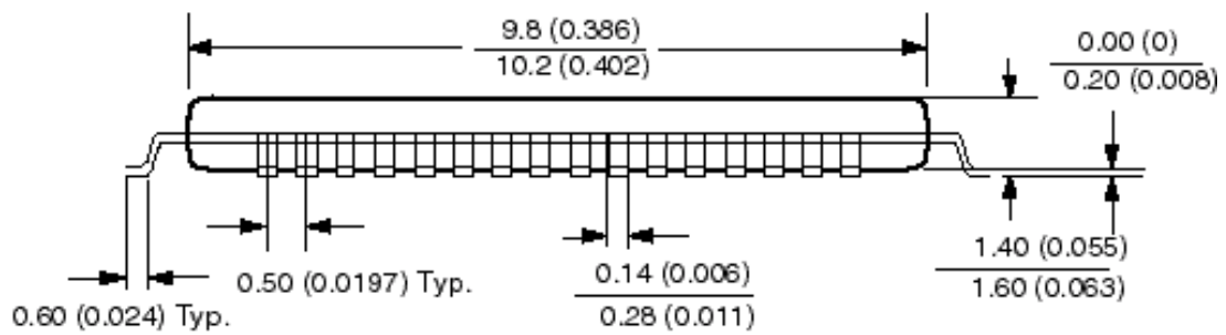
64-TQFP (JEDEC LQFP) Mechanical Specification
