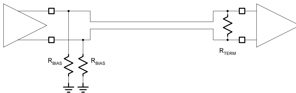
FIGURE 1. PECL INTERFACE
