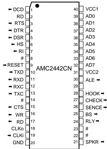
AMC2442CN Pinouts
