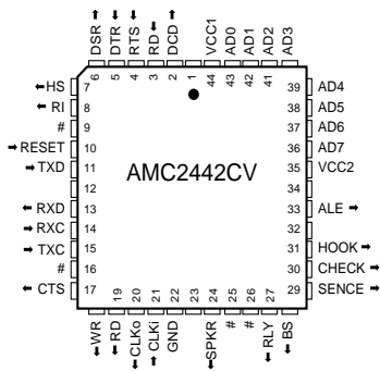
AMC2442CV Pinouts
