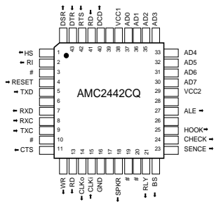
AMC2442CQ Pinouts
