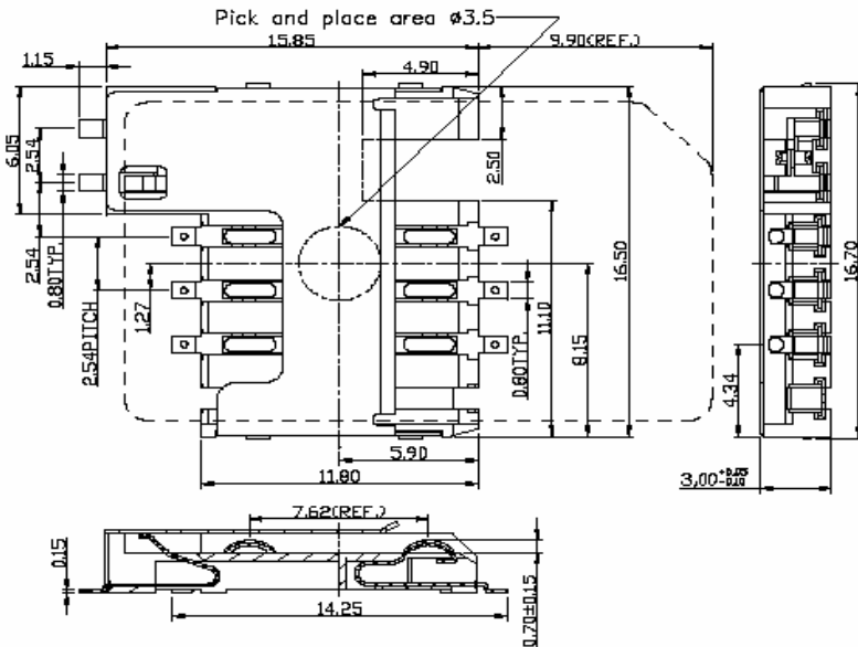
Unit: mm; Tolerances: \pm 0.15 mm Mechanical outline dimension
