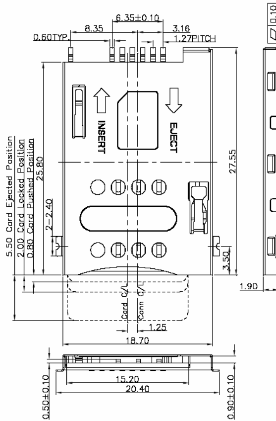
Unit: mm; Tolerances: ±0.15 mm Mechanical outline dimension
