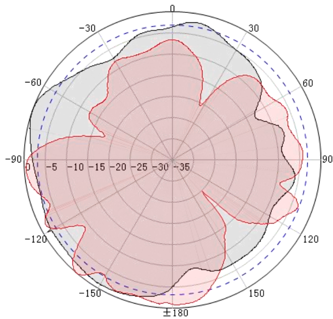
E-Plane @ 920MHz
